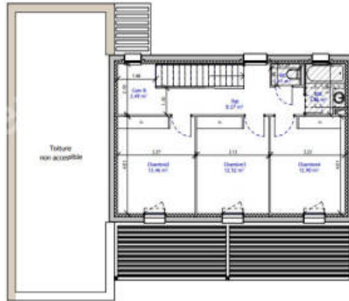
Plan R+1
